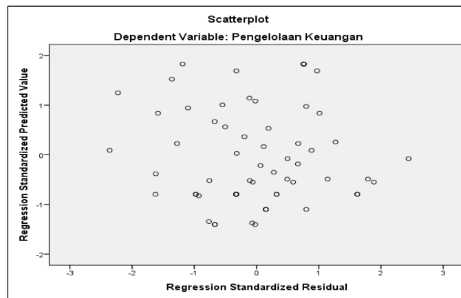
Gambar 3. Scatterplot
